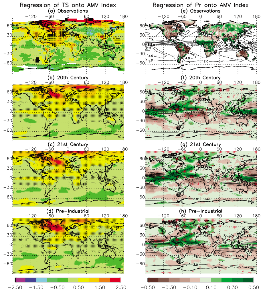
Figure 2. Global surface temperature regression onto the AMV indices for (a) observations, (b) 20th Century with A1b scenario, and (c) 21st Century with A1b scenario, and (d) Preindustrial CMIP3 model simulations. (e–h) Same as Figures 2a–2d, but for precipitation. Stippling in Figures 2a and 2e indicates 95% confidence level based on Monte Carlo test, in Figures 2b, 2c, 2f, and 2g indicates 18 out of 23 models showing the same sign regression coefficients, in Figures 2d and 2h indicates 16 out of 20 models showing the same sign regression coefficients. Contours in right panels are for climatological precipitation contoured at 2 mm/day intervals.
