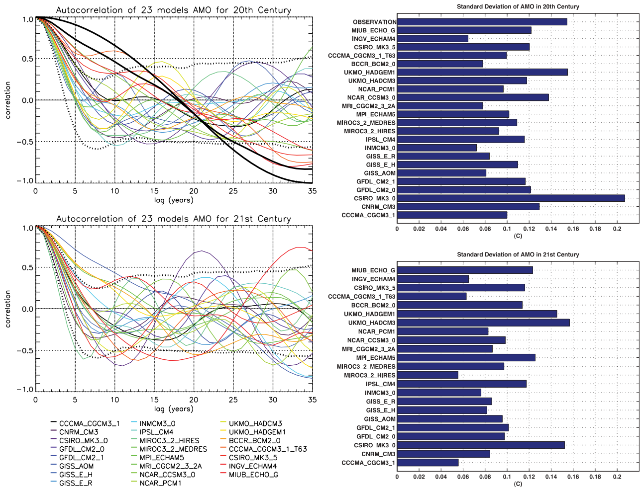
Figure 1. Autocorrelation of AMV indices in models (color lines) and observations (black line) with lags from zero to 35 years for (top left) 20th Century and (bottom left) 21st Century with A1b scenario. Black dot-dashed line is the auto-correlation when calculated for a perfect sine function with a period of 70 years, and the dotted black lines represent the 5% significance intervals at each lag based on autocorrelations of the filtered white noise time series. The keys for the color lines are indicated at the bottom on the left. (top right and bottom right) The corresponding amplitudes for the AMV indices.
