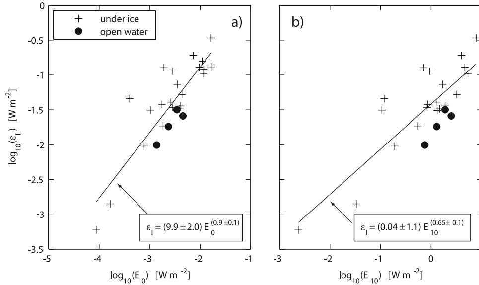
Figure 9. The dissipation integrated over the mixed layer, \varepsilon_1 , versus (a) under-ice energy flux rate, E_0 , (b) wind work at 10 m, E_{10} , for ice stations (crosses) and open water (solid circles). The upper 5–8 m of the dissipation profile not reliably measured by our sampling is approximated using LOW. The intercept and exponent of the linear fit are indicated with \pm standard errors.
