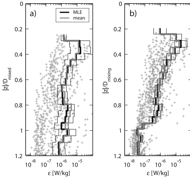
Figure 4. Observed dissipation profiles for the ice-covered stations of the survey, where the ordinate is the vertical distance from the ice, |z| , scaled (a) by the mixed layer depth, D_{\text{mixed}} , and (b) by the mixing layer depth, D_{\text{mixing}} . Presented are set-averaged 23 profiles (gray crosses), their arithmetic mean in 0.05 unit normalized distance bins (gray line), and the maximum likelihood estimate (MLE) values (black line). The MLE line agrees with that of the arithmetic mean within 95% confidence intervals.
