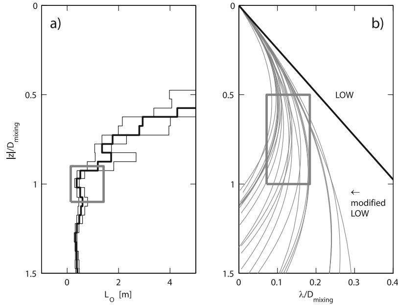
Figure 7. Profiles of (a) Ozmidov length scale L_O = (\varepsilon/N^3)^{1/2} MLE values (thick lines) and 95% confidence intervals (thin lines) and (b) mixing length scale \lambda normalized by the mixing layer depth for law of the wall (LOW, thick line) and modified law of the wall (shaded curves). In both Figures 7a and 7b, ordinate is the distance from ice scaled by D_{\text{mixing}} . Very large values of L_O in the nearly neutral stratification in the upper half of D_{\text{mixing}} are irrelevant and not shown. The horizontal extent of the shaded box in Figure 7a covers the total range of individual values for 23 mean profiles over |z|/D_{\text{mixing}} = 0.9-1.1 (vertical extent of the box) used in the calculation of the modified-LOW length scale. The horizontal extent of the box in Figure 7b is the range of maximum mixing length in the rotational outer boundary layer, \lambda_{\text{max}} \approx 0.03 u_{*0}/f , derived using local f and friction velocity for each MSS set (the vertical extent is arbitrary).
