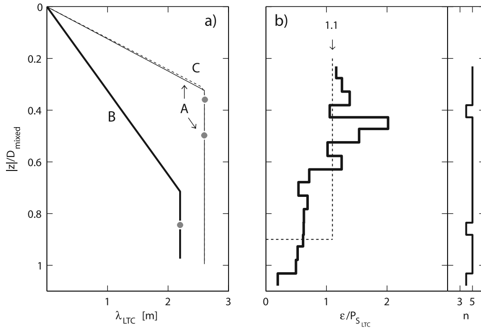
Figure 6. Vertical profiles of (a) mixing length for drift stations A (thin line), B (thick line), and C (dashed line) and (b) average dissipation scaled by the shear production, P_S , estimated using the local turbulence closure (LTC) model [McPhee, 1999]. Vertical distance from the ice is normalized by the mixed layer depth, D_{mixed} . Gray circles in Figure 6a mark |z|/D_{mixing} = 0.3 , for reference. The profiles are derived from station mean values in |z|/D_{mixed} = 0.05 unit bins, and the number of data points, n , used in averaging \epsilon is shown in the last panel. Scaled dissipation within |z|/D_{mixed} \leq 0.9 is 1.1 (vertical dashed line in Figure 6b).
