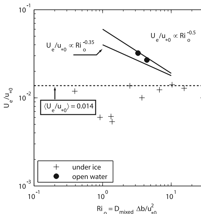
Figure 11. Normalized entrainment speed, U_e/u_{*0} , versus bulk Richardson number, \text{Ri}_o , derived from observations when the mixed layer was deepening. Drift stations do not show any apparent trend with \text{Ri}_o and scatter around a mean of 0.014. Relevant power laws reported in the literature are shown for reference. Two data points available from the ice-free station agree fairly well with the \text{Ri}_o^{-0.5} power law.
