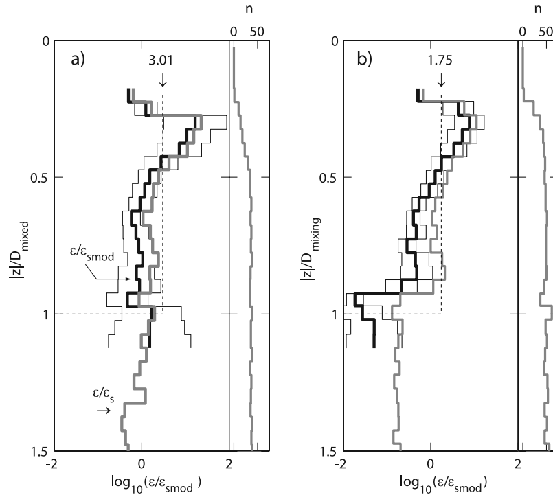
Figure 8. Profiles of dissipation rate \varepsilon normalized by the modified law of the wall \varepsilon_{\text{smod}} = u_{*0}^3/\lambda with \lambda from equation (5) (black lines), where the distance from ice |z| is scaled (a) by the mixed layer depth, D_{\text{mixed}} , and (b) by the mixing layer depth, D_{\text{mixing}} . The MLE values (black lines) and 95% confidence intervals are shown for |z|/D_{\text{mixing}} = 0.05 bins. There are typically \sim 50 data points, n , averaged in each normalized depth bin of the lower half of the mixed and mixing layers (narrow adjacent panels). The average of the standard LOW scaling (over both cases of ice relative speed in Figure 5) is shown for reference (gray lines).
