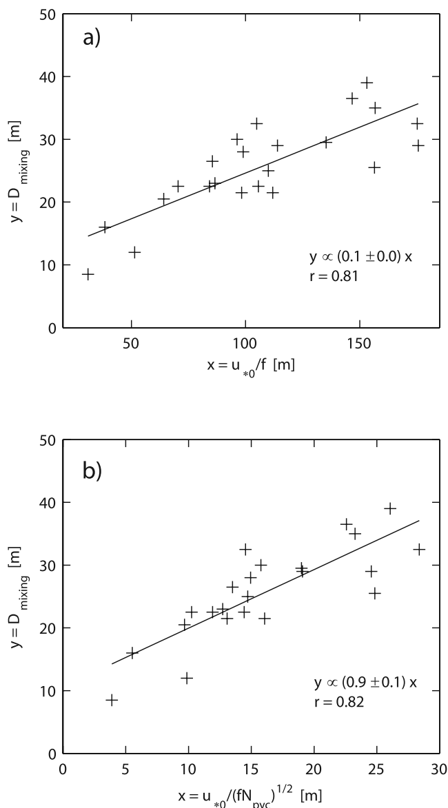
Figure 10. Regression of mixing layer depth, D_{\text{mixing}} , against (a) outer neutral planetary length scale, u_{*0}/f , and (b) stratified planetary length scale, u_{*0}/(fN_{\text{pyc}})^{1/2} . The slope ( \pm standard error) of the linear least squares fit (with nonzero intercept) is indicated together with the correlation coefficient, r . When intercept is set to zero slopes are 0.23 ( r = 0.65 ) and 1.5 ( r = 0.62 ) for Figure 10a and 10b, respectively.
