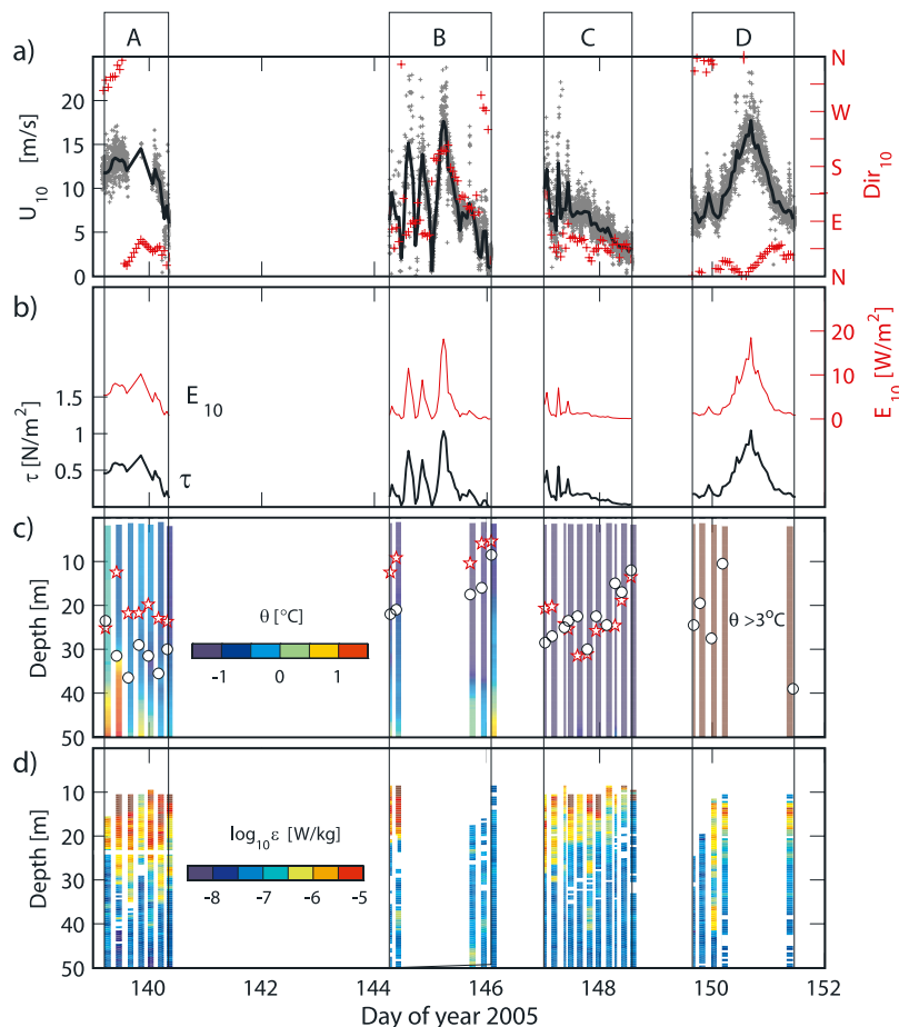
Figure 3. Overview of along-track (a) wind speed, U_{10} , and direction, (b) wind stress, \tau , and work, E_{10} , MSS-derived set-averaged color-coded profile of (c) potential temperature, \theta , and (d) dissipation, \varepsilon . Wind data are recorded at \sim 10 m from the ship weather station. The 1-min wind velocity record (speed shown as gray crosses in Figure 3a) are hourly vector-averaged (black line in Figure 3a), interpolated for missing data prior to calculation of direction, stress, and wind work. Time series cover varying geographic locations (Figure 1). The duration of occupation of the stations is bounded by vertical lines with stations' names indicated at top. Station D is in open water with temperature > 3 °C in the upper 50 m. In Figure 3c, open circles are the mixing layer depth, whereas red stars are the mixed layer depth. The typical duration of each MSS set is about 1 hour; however, the width of the color-coded columns in Figure 3c and 3d are arbitrary, \sim 3 hours, for clarity.
