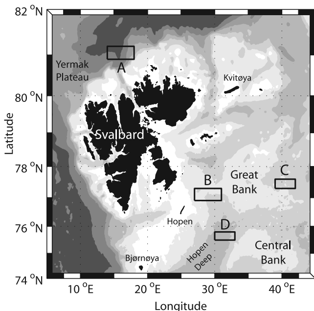
Figure 1. Location map of the study site with place names and occupied stations (A, B, C, and D) indicated by boxes covering the approximate spatial extent of each drift. The isobaths are 100, 200, 300, 500, 1000, and 2000 m.
