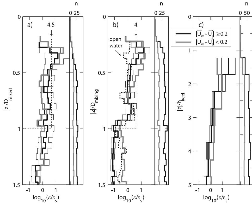
Figure 5. Vertical profiles of dissipation normalized by stress scaling, \varepsilon_s = u_{*0}^3/\kappa|z| , where the vertical distance from the ice, |z| , is scaled (a) by the mixed layer depth, D_{\text{mixed}} , (b) by the mixing layer depth, D_{\text{mixing}} , and (c) by the keel height, h_{\text{keel}} . The profiles are presented as MLE values over the number of data points, n (shown in narrow adjacent panels), in normalized depth bins (of length equal to 0.05 for Figures 5a and 5b and 0.5 for Figure 5c). The conditions when the magnitude of ice-relative velocity was greater than (black lines) and less than (gray lines) 0.2 m/s are shown separately. The 95% confidence intervals are given for only one profile, for clarity. The average values (over all values of ice relative speed) for the normalized depth \leq 1 are indicated in Figures 5a and 5b. The dashed line in Figure 5b is the profile derived for the open water station D, shown for reference.
