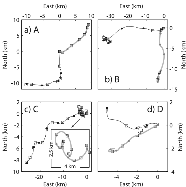
Figure 2. (a–d) Progressive vector diagrams derived from 12-hour smoothed ship velocity (black lines, representative of the ice drift in Figure 2a–2c) and depth-averaged current (thick gray lines). Solid circles are placed at 6-hour intervals; the solid squares are placed at the mean time of each microstructure profiler (MSS) set. The diagrams cover the durations identified in Figure 3, except that Figure 2d terminates \sim 24 hours before the last MSS set. The depth-averaged current in Figure 2c is enlarged in a box of 4 \text{ km} \times 2.5 \text{ km} to show the near-inertial period loops.
