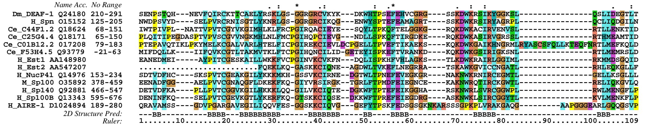
Fig 1b. Alignment of SAND domains.
