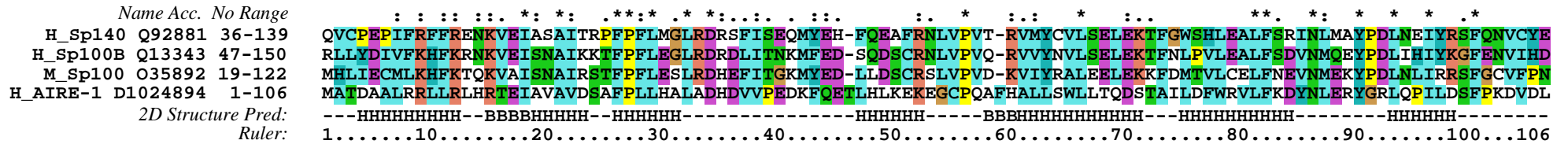
Fig 1a. Alignment of N-terminal domains from Sp100 group proteins
