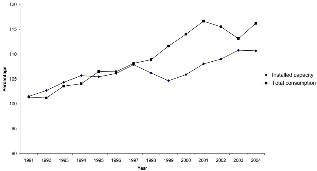
Fig. 2. Development of installed capacity and total electricity consumption in the Nordic countries relative to year 1991 (Source: Nordel Annual Reports)
