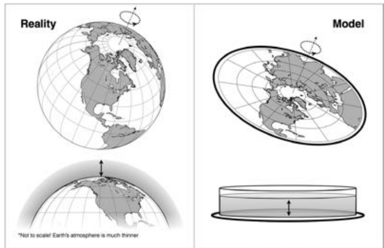
FIG. 3. Schematic used on the DIYnamics website and other materials. The graphical depiction of projecting the spherical Earth onto a flat surface helps students recognize the utility of a rotating tank of water as a model for planetary fluids. An analogous schematic was presented by Read et al. (1998).
