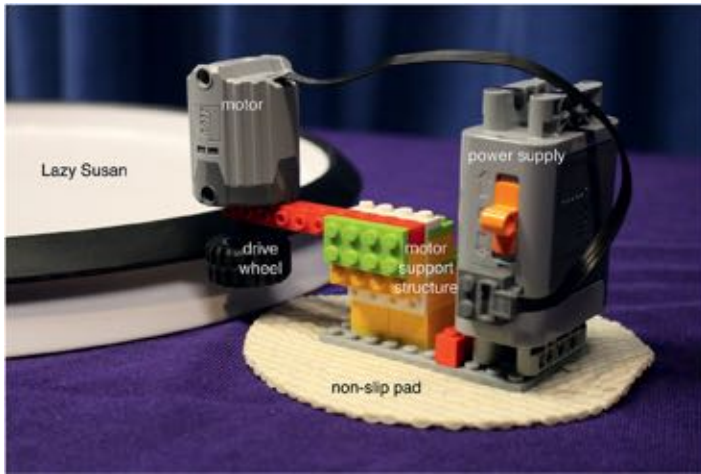
FIG. 1. Photograph of the DIY dynamics rotating table platform with key components labeled. Video instructions are available online ( https://youtu.be/rvF6UA08vPA ).
