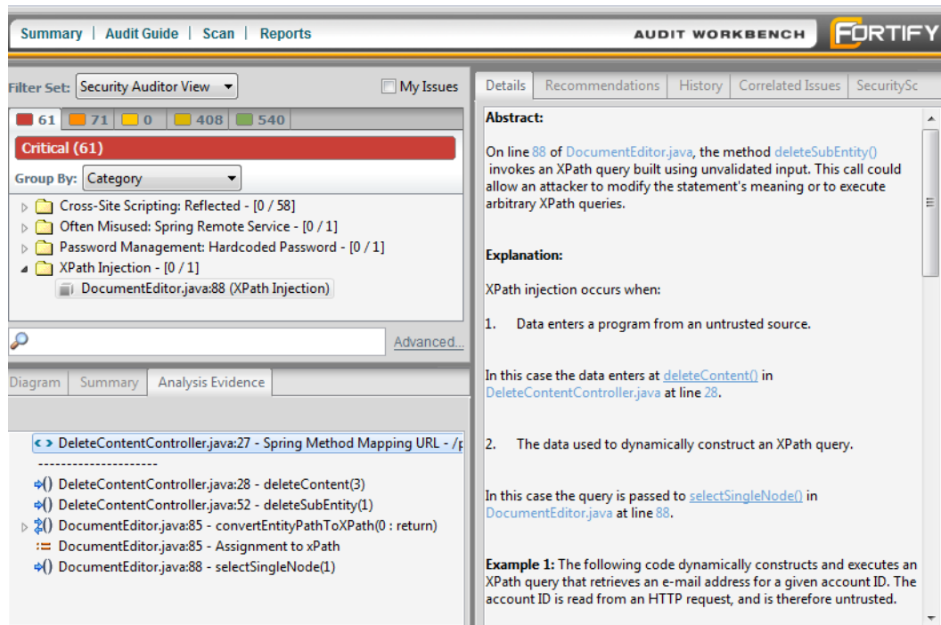
Figur 4.6: Fortify SCA
